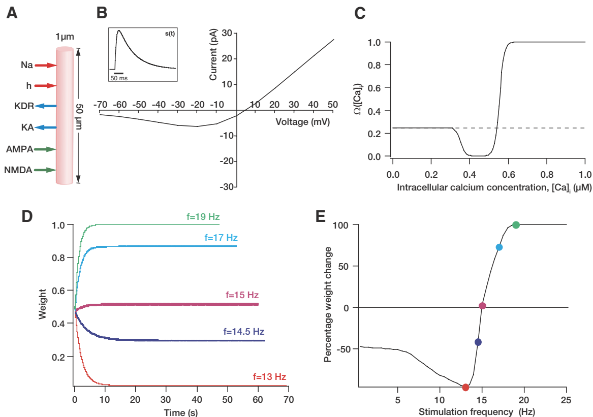
FIG. 1. Illustration of the basics of our model. A : schematic of the single compartment model used in this study. The various ligand- and voltage-gated channels used in the model are depicted as arrows. B : properties of N -methyl-D-aspartate receptor (NMDAR) current used in the model. The current through the receptor as a function of membrane voltage shows the magnesium dependent voltage block at hyperpolarized voltages. Inset : time course of a typical NMDAR excitatory postsynaptic potential (EPSP). C : functional form of the plasticity-regulating \Omega -function plotted for various concentrations of intracellular calcium. D : evolution of weight w , when the model was stimulated with 900 pulses of multiple frequencies, plotted as a function of time. It may be noted that the evolution approximates an exponential. The color codes for various frequencies translate to E as well. Because 900 pulses of a low-frequency stimulus ended later than 900 pulses of a high-frequency stimulus, the endpoints are variable. It may be noted that at the end of the stimulus protocol, the weight parameter increased (potentiation) for frequencies that are approximately > 15 Hz while decreasing (depression) for frequencies lesser than that value. E : plot obtained by tracking percentage change in weight w after 900 pulses of stimulus at various frequencies. The colored dots represent the values obtained from D for corresponding frequencies.
